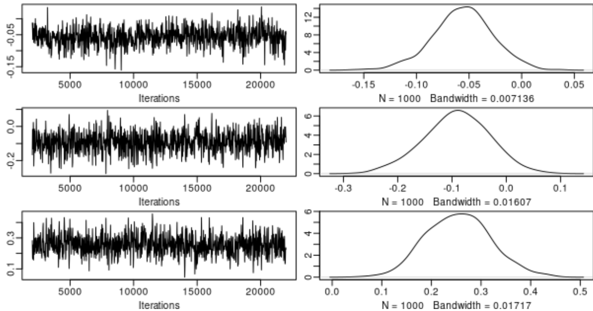
Figure 2: Trace plots and estimated kernel densities of posterior draws from p(\beta | \mathbf{y}) .
